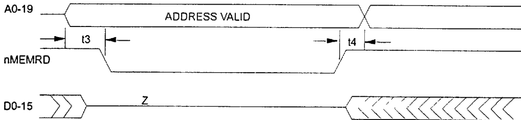
FIGURE 28 - 8-BIT MODE REGISTER CYCLES
