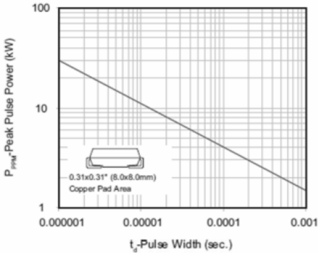
Figure 1 - Peak Pulse Power Rating
