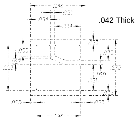
Figure 8. Package Dimensions
