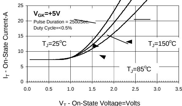
Figure 1. On-State Characteristics
