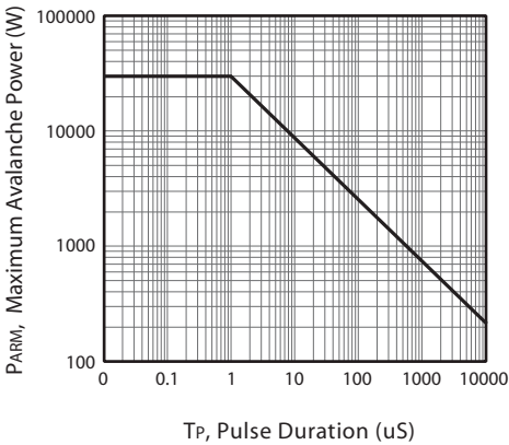
Figure 6. Maximum Avalanche Power Curve
