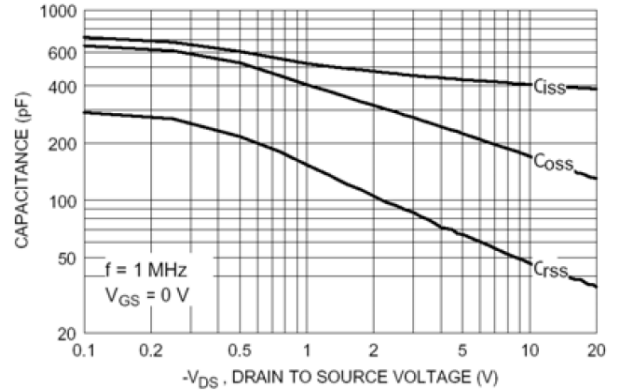
Figure 8. Capacitance Characteristics.
