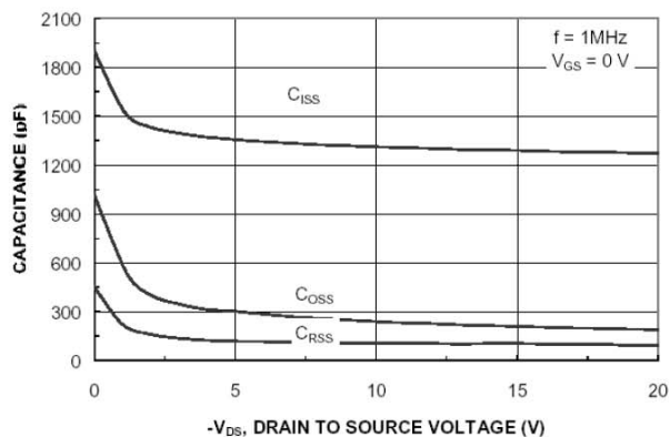
Figure 8. Capacitance Characteristic
