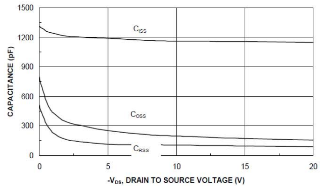
Figure 4. Capacitance
