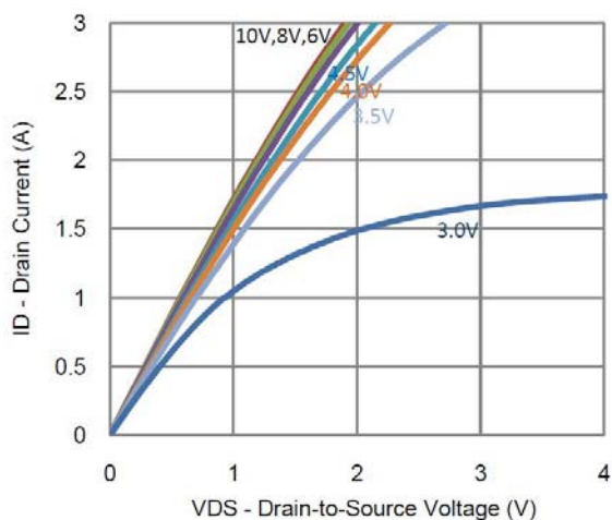
5. Output Characteristics
