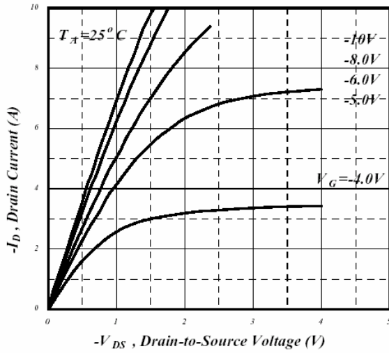
Characteristics Curve
