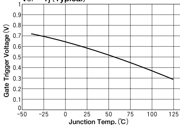
V_{GT} - T_j (Typical)
