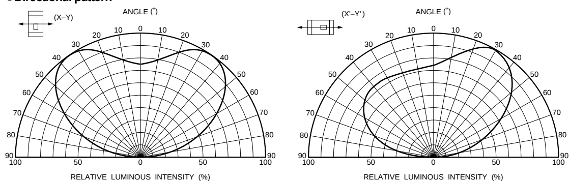
Fig.1 Directional pattern
