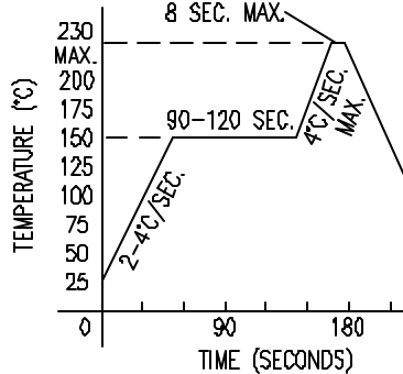
REFLOW PROFILE
