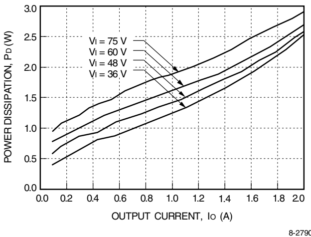
Figure 9. SMLW010A Typical Power Dissipation vs. Normalized Output Current at TA = 25 °C
