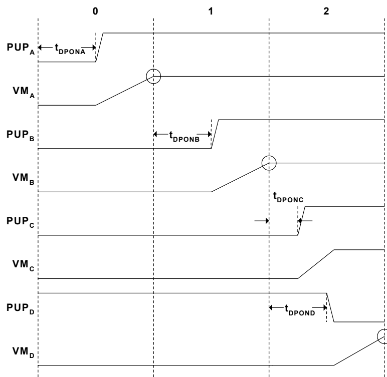
Figure 5 - The SMM465 cascade sequencing the supplies on and then monitoring for fault conditions.
