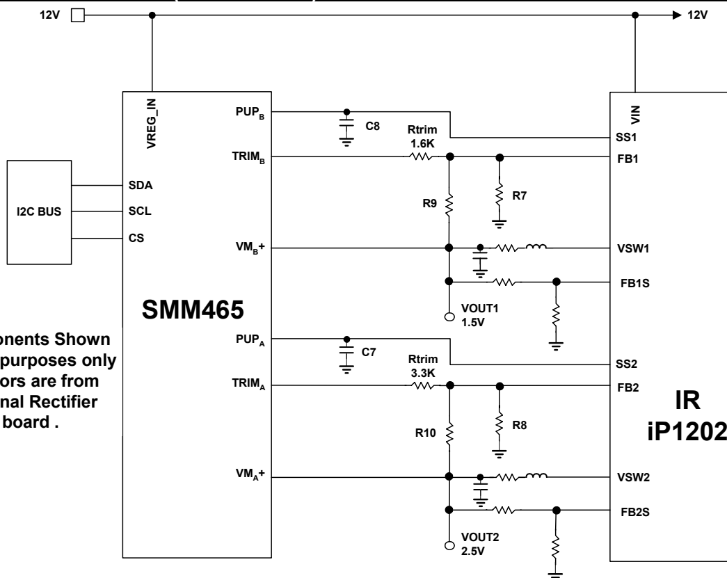
Figure 12 – The SMM465 can be used to sequence and control discrete DC switching regulators. The ADOC function sets the output voltage of the IR iP1202 Regulator through the FBX feedback pins. Accuracy is improved even under full load, essentially acting as a “SENSE” pin. The sequence function is applied through the iP1202 SSX soft start pins.
