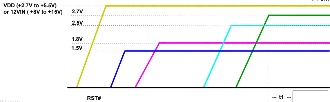
Figure 2 – Example Power Supply Sequencing and System Start-up Initialization using the SMM465. Any order of supply sequencing can be applied using the SMM465. Power supply ordering, trimming and Active DC control allows supply cascade sequencing, automatic level adjustment, margin testing and reset control.
