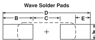
FIGURE 4 - RECOMMENDED MOUNTING PAD GEOMETRIES in inches (millimeters)
