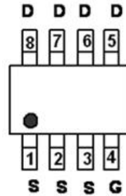
Pin Assignments
