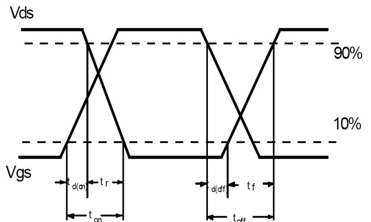
Switching Waveforms:
