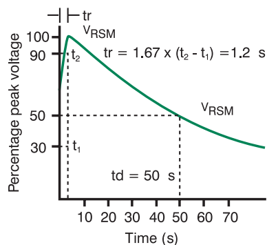
1.2/50 \mu S IMPULSE DISCHARGE VOLTAGE WAVESHAP
