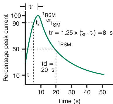
8/20 \mu S IMPULSE DISCHARGE CURRENT WAVESHAP
