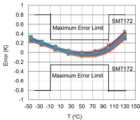
Accuracy vs. Temperature (TO18 V_{\text{CC}}=5\text{V} )
