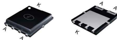
Package: POWER QFN5x6
