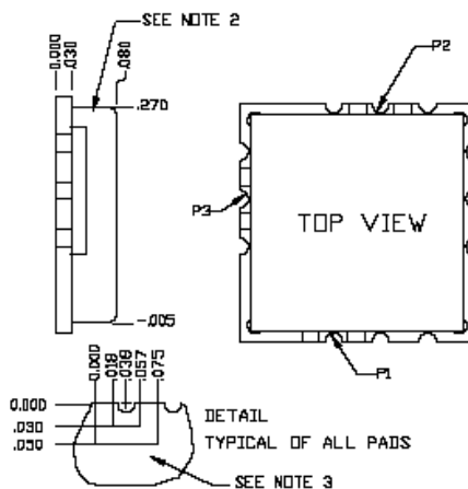
PHYSICAL DIMENSIONS
