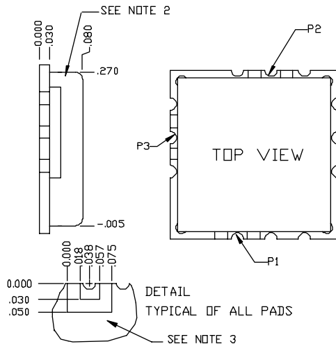
PHYSICAL DIMENSIONS
