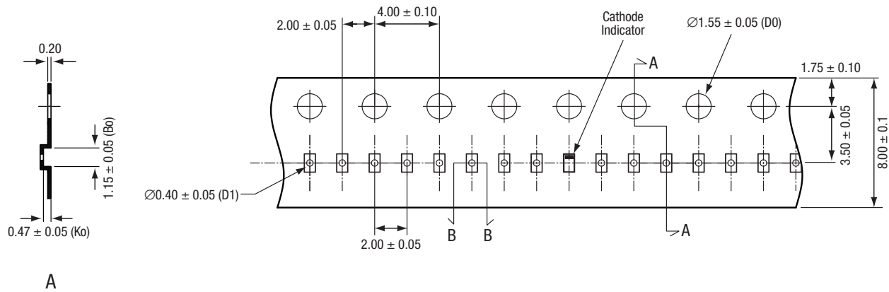
Figure 4. SOD-882 Package Dimensions
