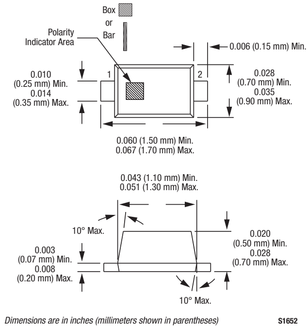
Figure 4. SMV2025-079LF Package Dimensions (SC-79)
