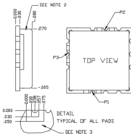
PHYSICAL DIMENSIONS
