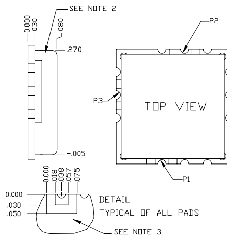
PHYSICAL DIMENSIONS
