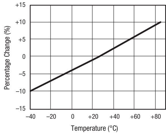
Figure 2. Relative Series Resistance Change vs Temperature @ 500 MHz
