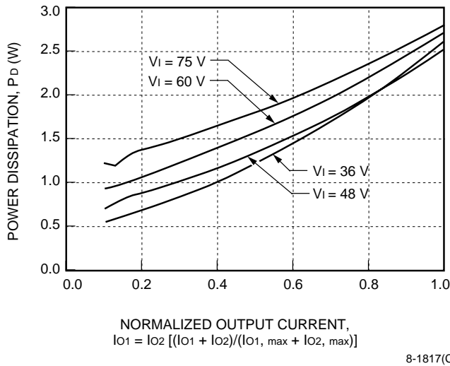
Figure 16. SMW010AJ, BK, CL Typical Power Dissipation vs. Normalized Output Current at T_c = 25^\circ\text{C}
