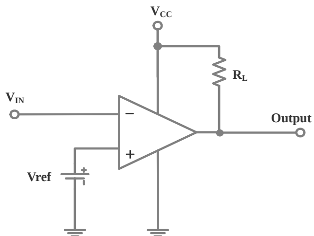
Basic Comparator
