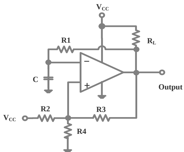
Square-wave Oscillator
