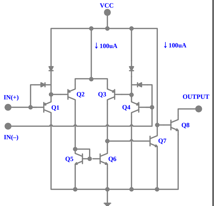
Equivalent Circuit
