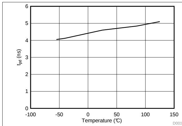
Figure 1. t_{pd} vs Temperature at 3.3-V V_{CC}
