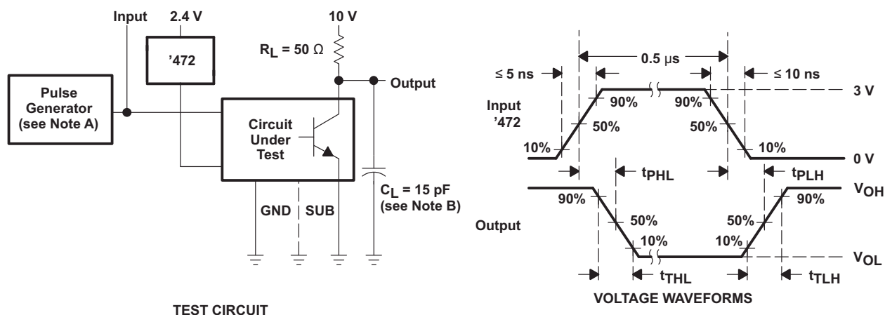
Figure 2. Switching Times
