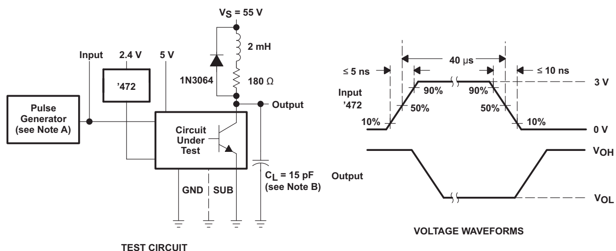
Figure 2. Switching Times
