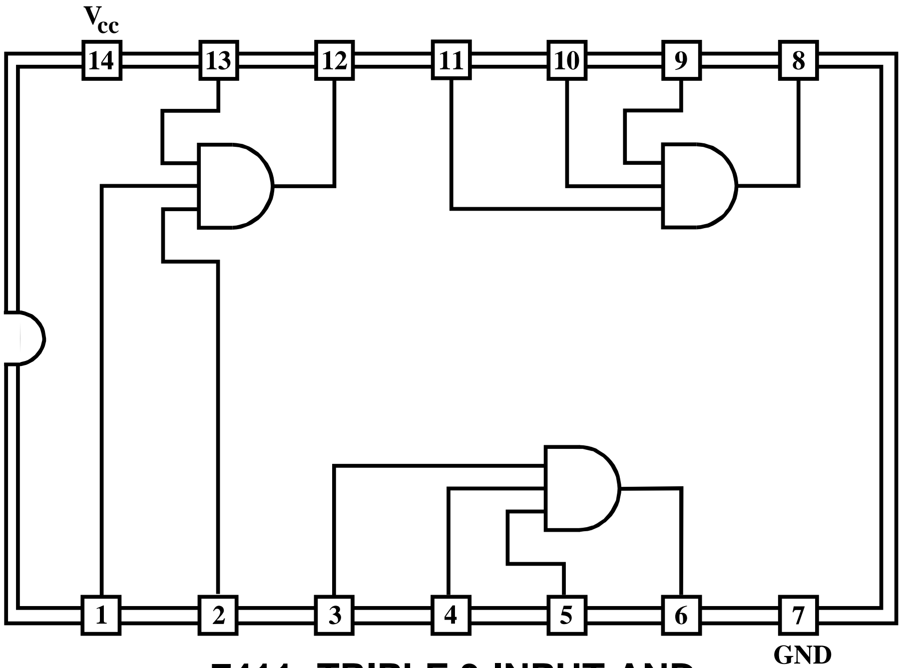
7411: TRIPLE 3-INPUT AND
