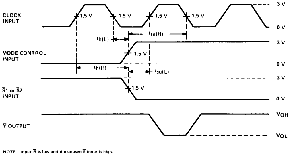
FIGURE 5—ENABLING SINGLE PULSE
