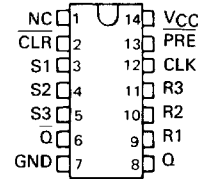
SN54L71 ... J PACKAGE (TOP VIEW)
