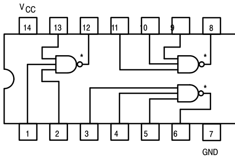
* OPEN COLLECTOR OUTPUTS
