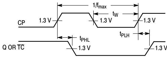
Figure 1. Clock to Output Delays, Count Frequency, and Clock Pulse Width
