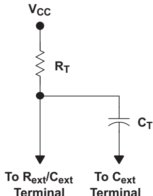
Figure 12. Timing-Component Connections
