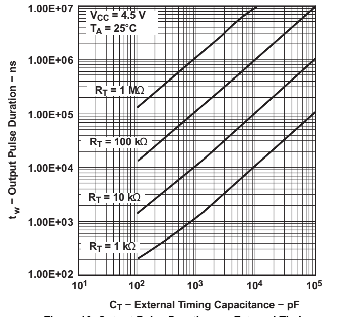
Figure 16. Output Pulse Duration vs. External Timing Capacitance
