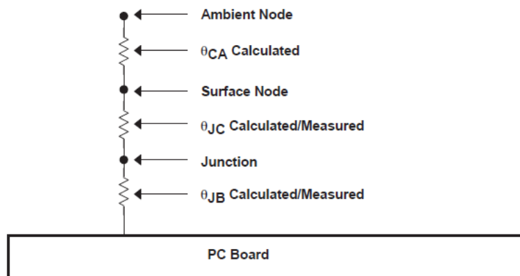
Figure 7-2. Thermal Resistance
