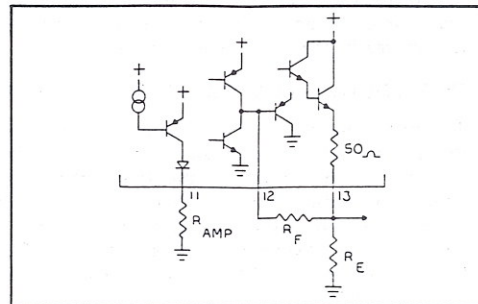
Operational Amplifier Internal Input Circuitry
