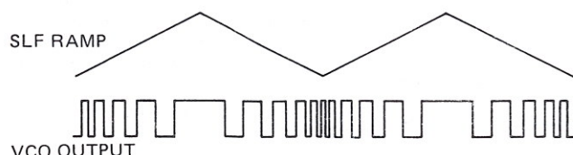
VCO FM output
