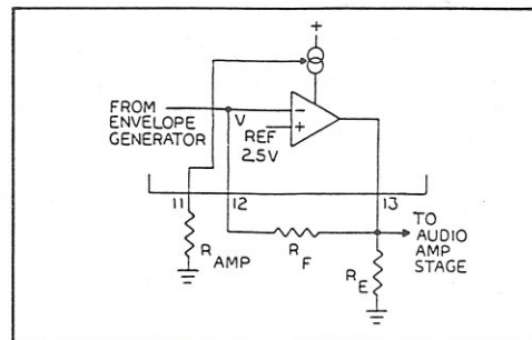
Operational Amplifier
