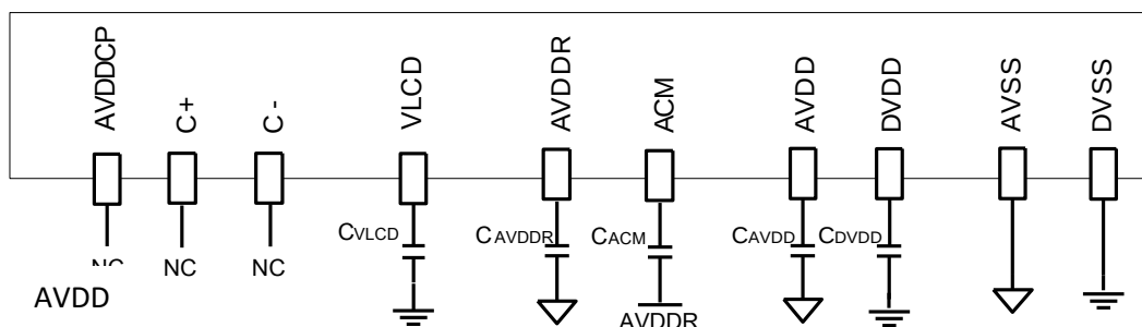
Analog Capacitor Connection (Charge pump disable):
