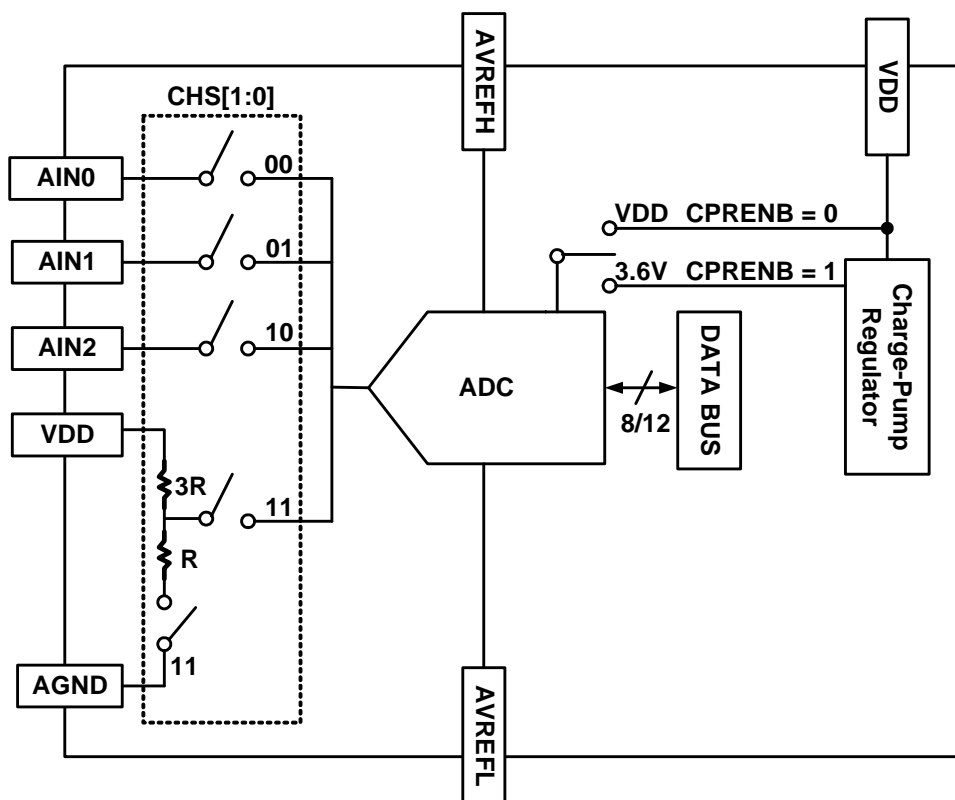
Figure 13-1. AD Converter Block Diagram
