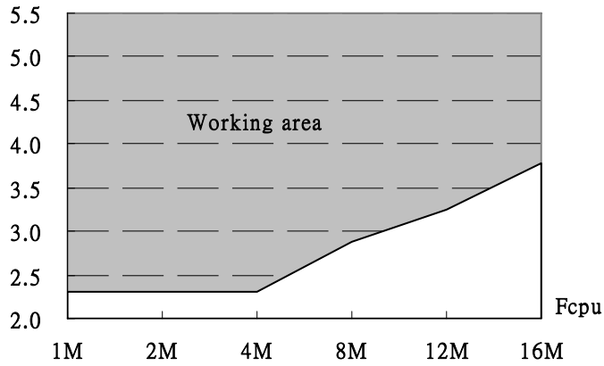
Working Voltage vs. Frequency (Noise Filter Disable、25°C)
