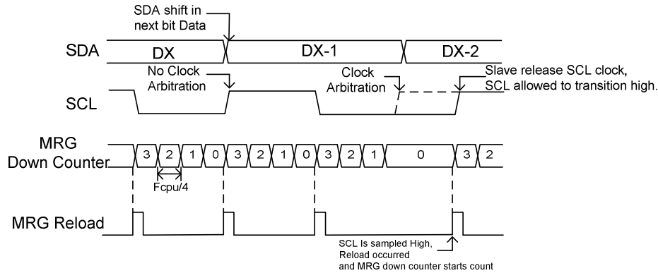
MRG Timing Diagram with and without Clock Arbitration (MSPADDR=0x03)
