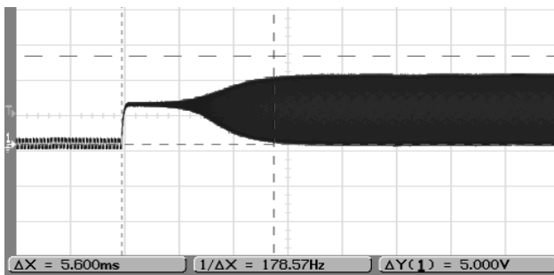
32768Hz Crystal
