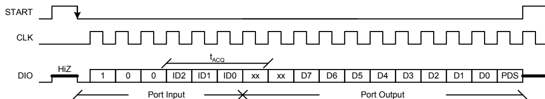
Figure5 The timing diagram of ADC reading
