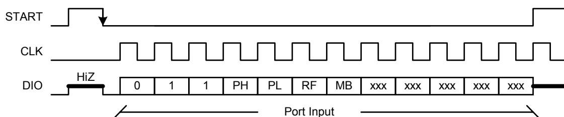
Figure4 The timing diagram of control registers setting
