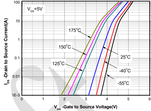
Transfer Characteristics (4)
