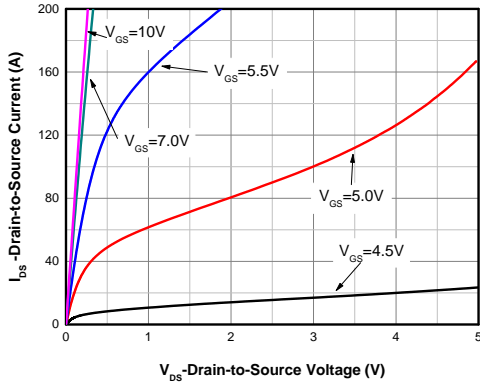
Output Characteristics (4) (4)
