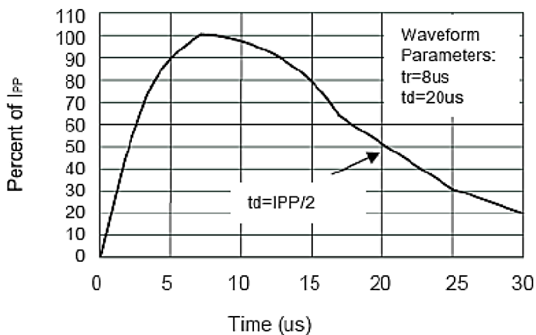
Pulse Waveform
