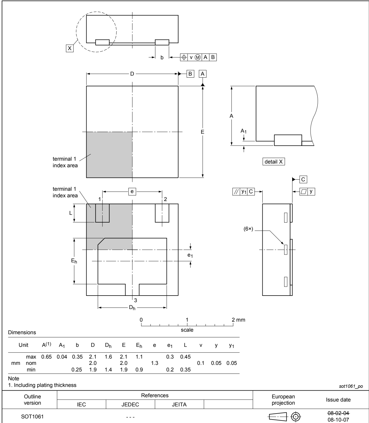
Fig. 1. Package outline DFN2020-3 (SOT1061)
