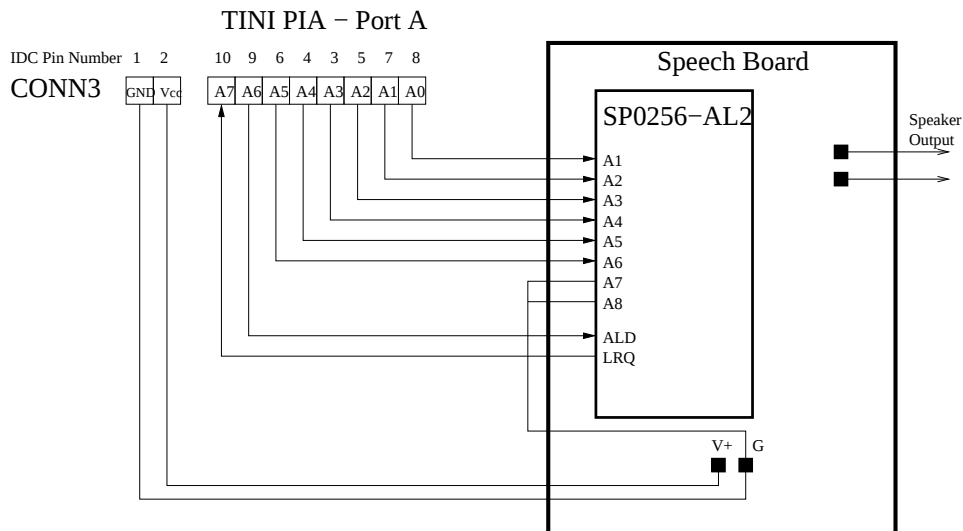
Figure 1: SP0256 Interface
