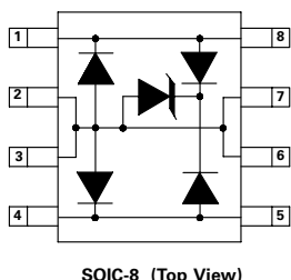
SOIC-8 (Top View)
