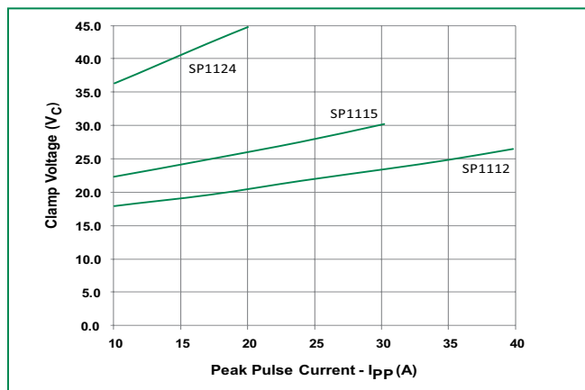
SP1112, SP1115, SP1124 Clamping voltage vs. I_{pp} for 8/20 \mu s waveshape
