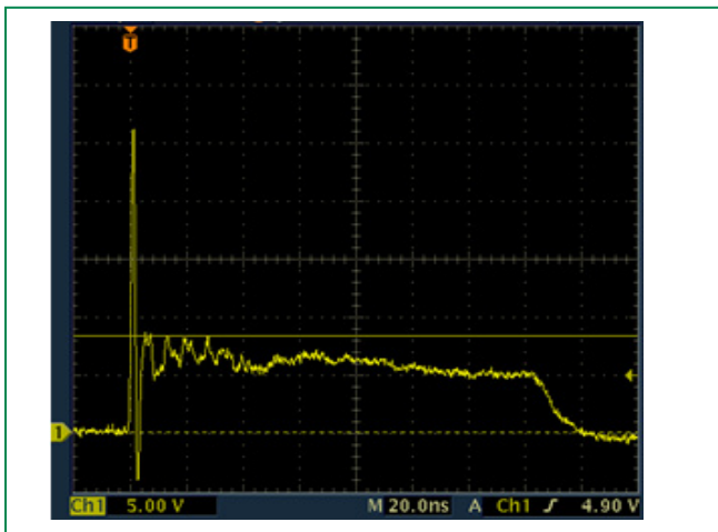
SP1105S IEC 61000 –4–2 +8 kV Contact ESD Clamping Voltage
