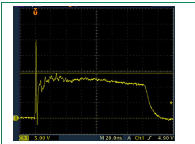
SP1112 IEC 61000 –4–2 +8 kV Contact ESD Clamping Voltage
