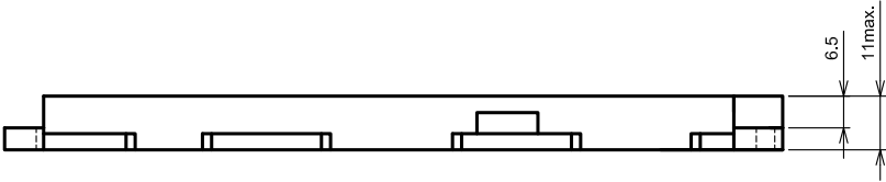
FRONT VIEW
